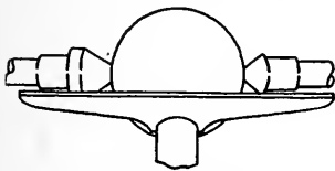
FIG. 329. TURNING SPHERE BETWEEN CENTERS.
